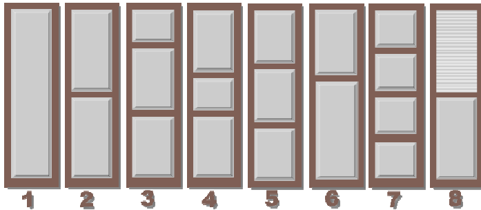
Colonial Raised Panel Shutter Specifications
